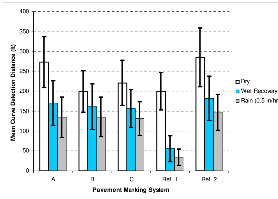
Figure 17. Mean Taper Detection Distance as a function of Pavement Marking System and Environmental Condition.
