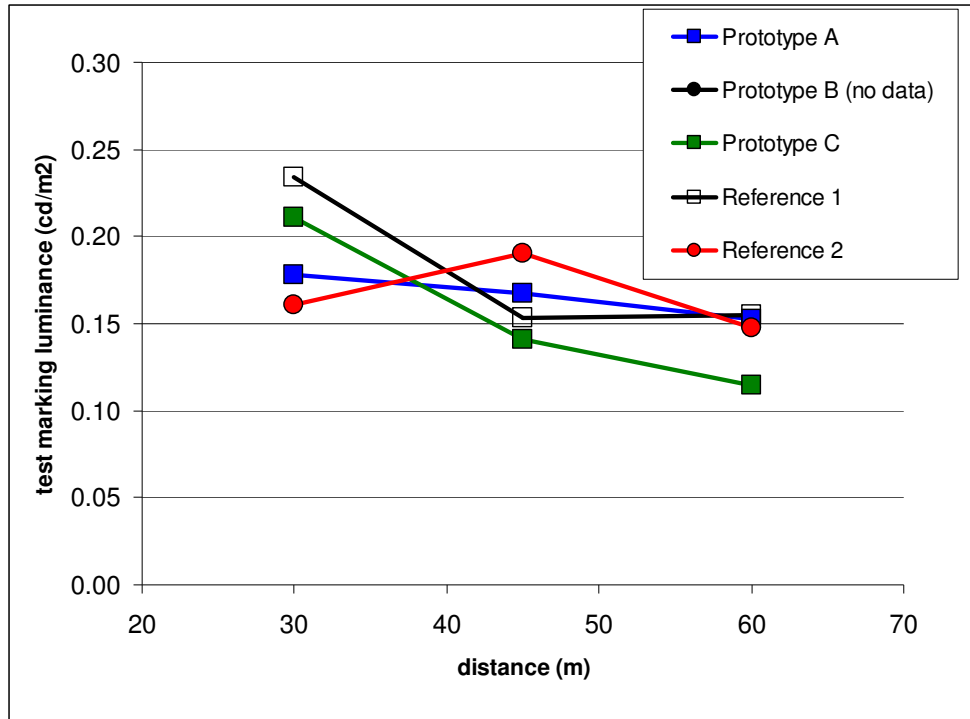
Figure 28. Luminance of the roadway surface adjacent to the test marking from the driver point-of-view through the windshield as a function of distance (rain conditions).
