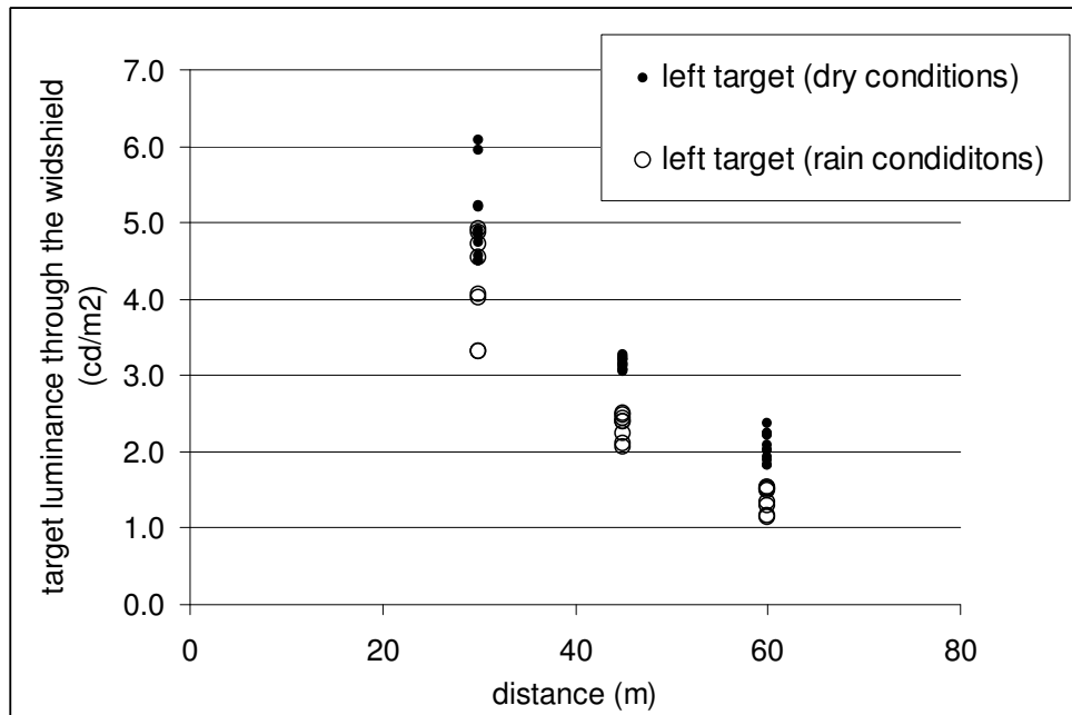
Figure 26. Diffuse target luminance from the driver point-of-view through the windshield as a function of distance, position on the road and conditions (dry versus rain conditions).
