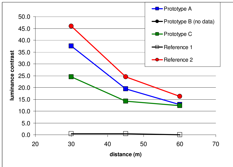
Figure 29. Luminance contrast between the test marking and the adjacent roadway surface as a function of distance (rain conditions, Contrast = (Lmarking-Lroad)/Lroad).
