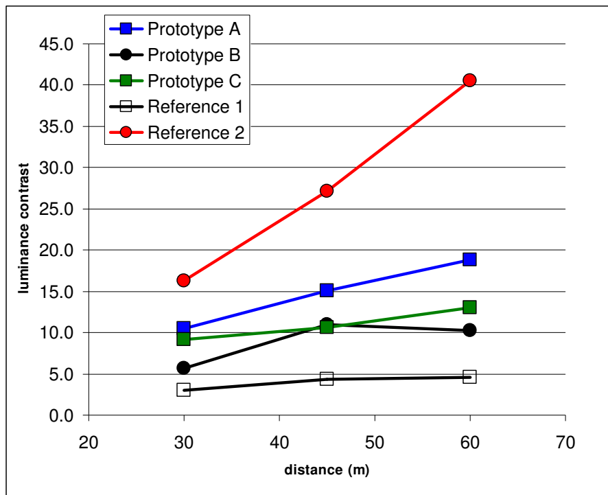
Figure 25. Luminance contrast between the test marking and the adjacent roadway surface as a function of distance (dry conditions, Contrast = (L_{\text{marking}} - L_{\text{road}}) / L_{\text{road}} ).
