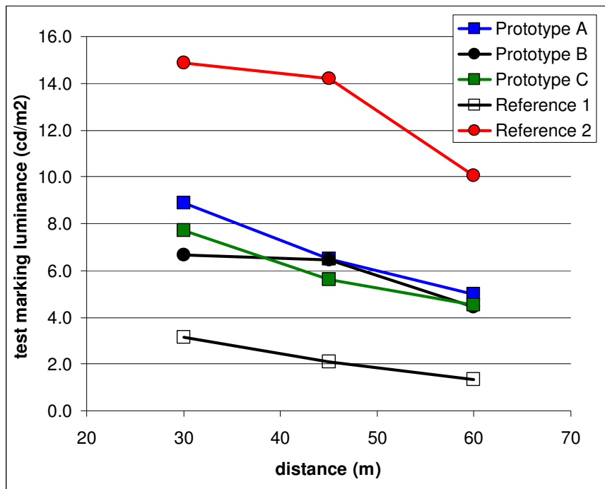
Figure 23. Test marking luminance from the driver point-of-view through the windshield as a function of distance (dry conditions).
