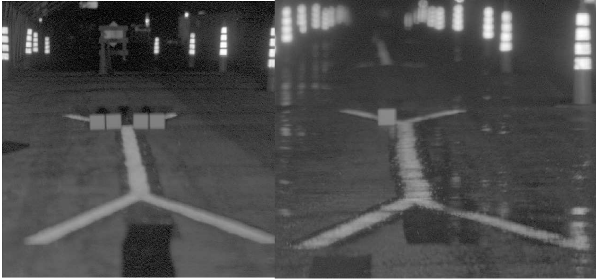
Figure 30. Screen captures from imaging photometer showing Prototype A at a distance of 45m under dry (left) and rain (right) conditions.
