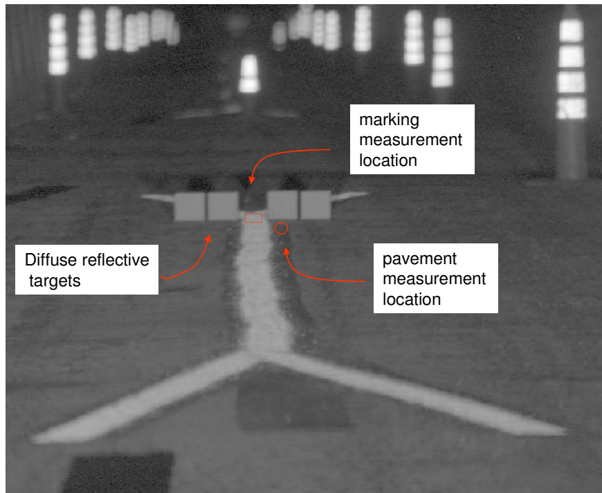
Figure 18. Screen capture from imaging photometer showing the locations of the reference luminance measurement location and set-up for the diffuse reflectance targets under dry conditions.
