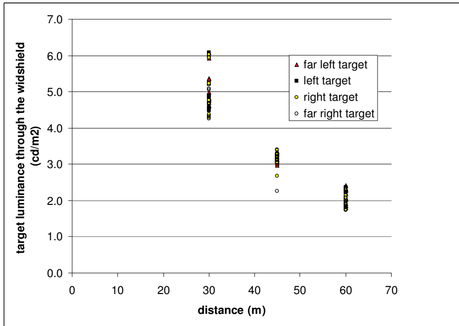
Figure 21. Diffuse target luminance from the driver point-of-view through the windshield as a function of distance and position on the road (dry conditions).
