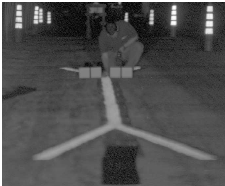
Figure 19. Illustration of illuminance measurement using the handheld illuminance meter.
