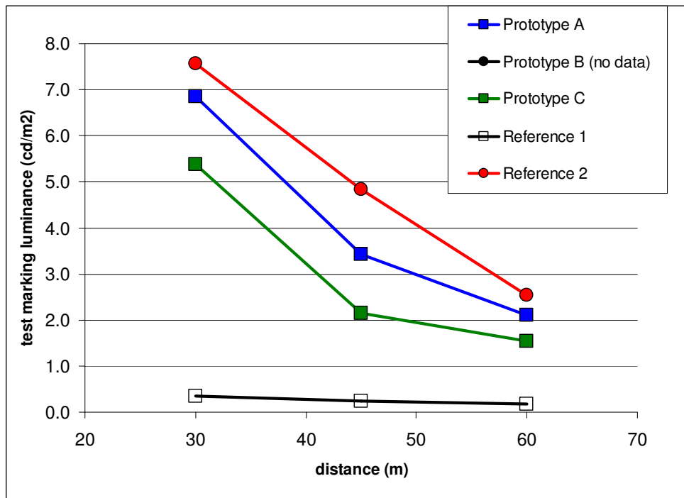
Figure 27. Test marking luminance from the driver point-of-view through the windshield as a function of distance (rain conditions).
