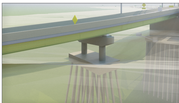
Images like these from the project’s as-built 3D model show the relationship between drainage structures, piles, pile cap, and pier signage structure. Source: NYSDOT
