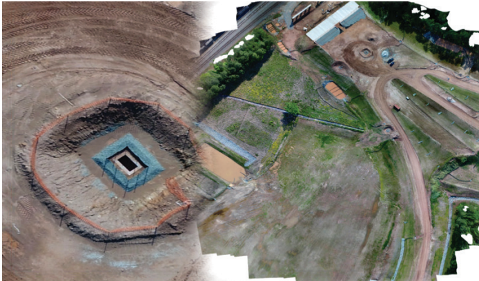
Figure 6. UAS orthograph images
